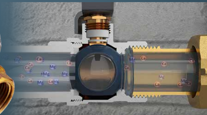
Ball is covered with nanoceramics - avoidance of limescale deposits disturbing the operation of the valve.
