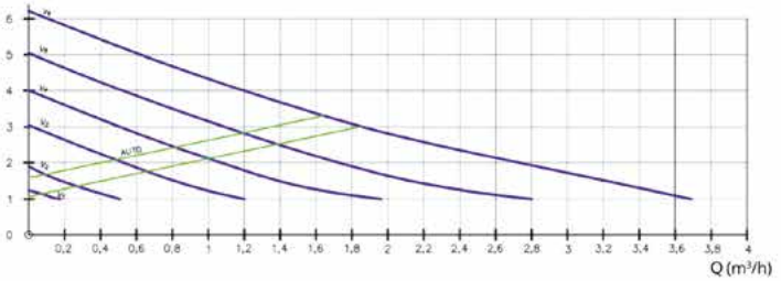
H(m) CI-HELIO 25/60-130, CI-HELIO 25/60-180,
