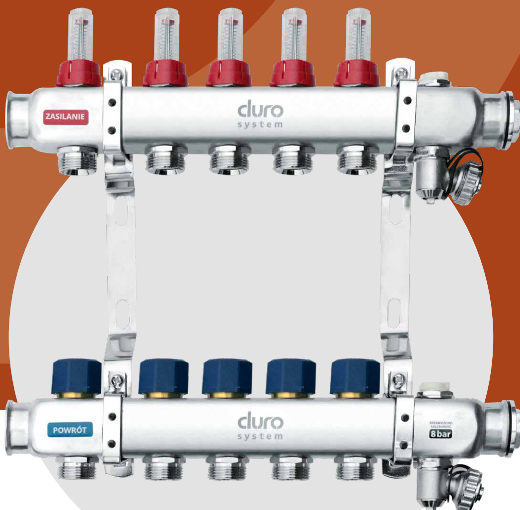
Floor heating manifolds Duro system
