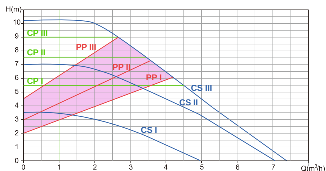
CI-SELEN 25/100-180
