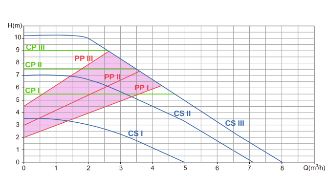
CI-SELEN 32/100-180
