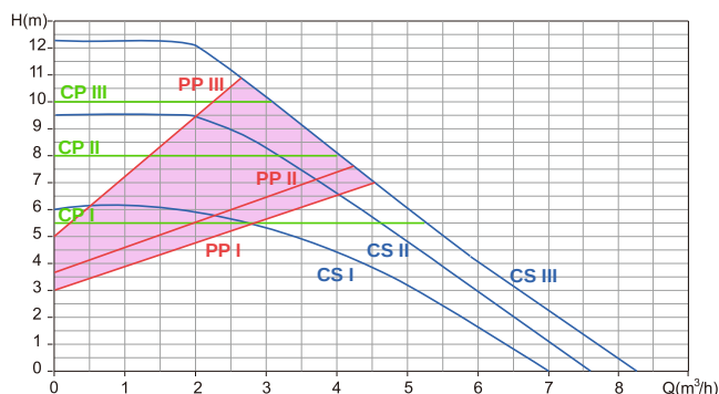
CI-SELEN 25/120-180
