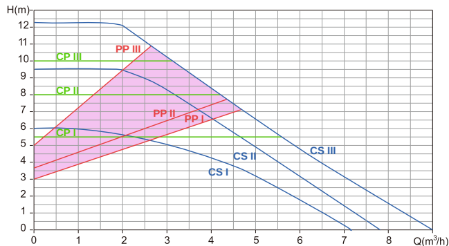
CI-SELEN 32/120-180
