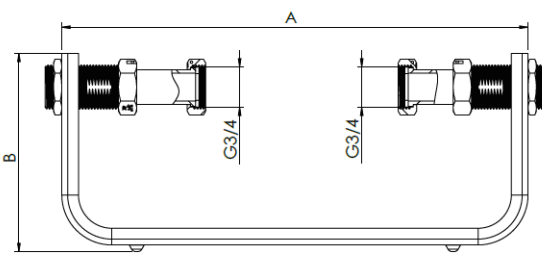
CA/KW-DN15
