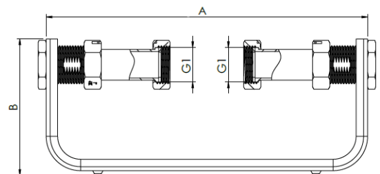
CA/KW-DN20
